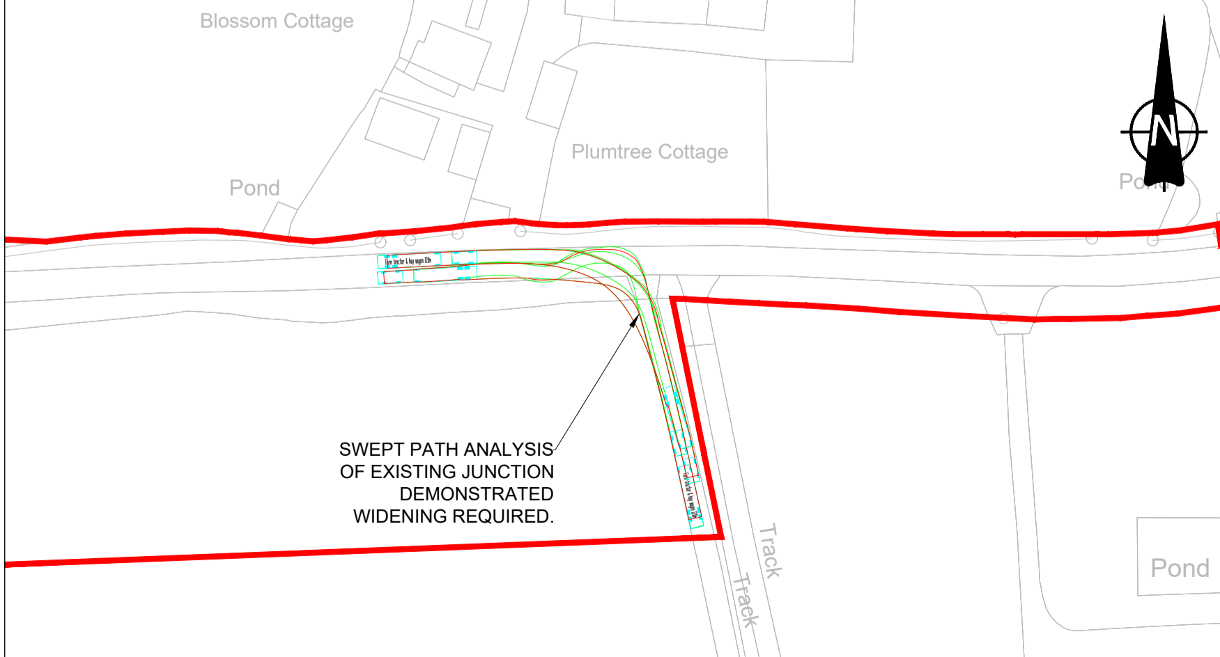
INSET A: FARM TRACTOR AND TRAILOR MANOEUVRES (NO JUNCTION IMPROVEMENTS), HEADING OUT OF ACCESS, LEFT TURN ONTO MOSS ROAD. HEADING EAST ON MOSS ROAD, RIGHT TURN INTO ACCESS - SCALE 1:1000
