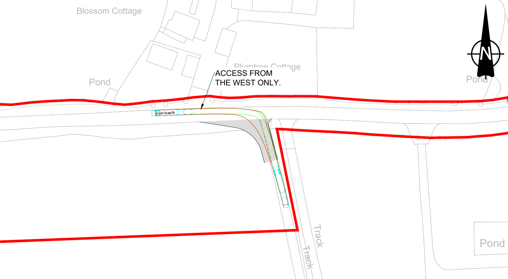
INSET B: FARM TRACTOR AND TRAILOR MANOEUVRE, HEADING EAST ON MOSS ROAD, RIGHT TURN INTO ACCESS - SCALE 1:1000
